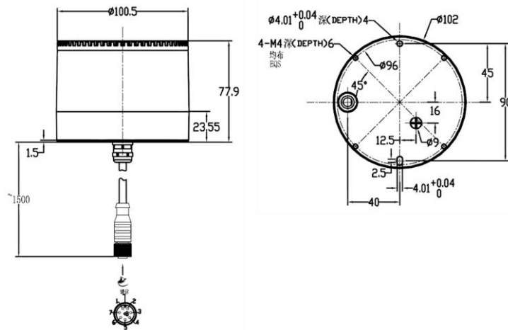
Figure 1.4 C8 Dimensions 1 (cable interface on the bottom) (unit: mm)
