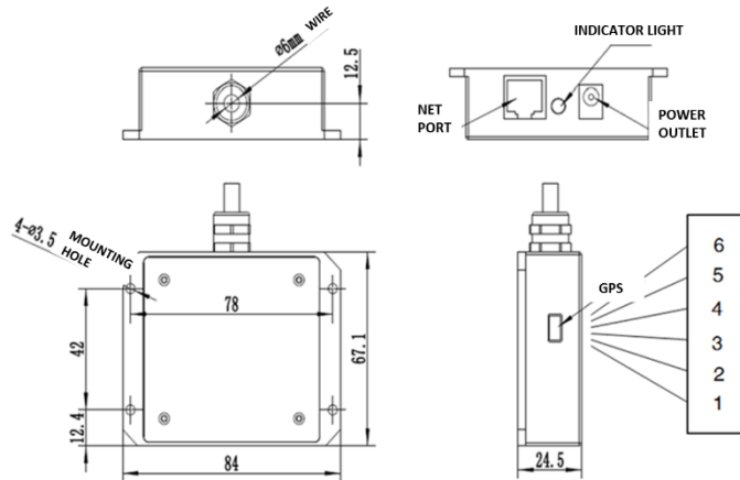
Figure 2.7 Interface Box
