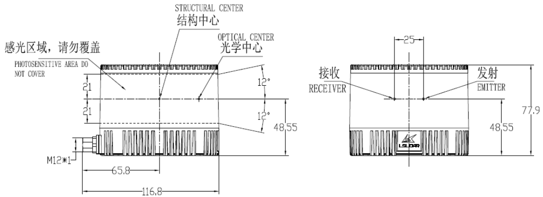
Figure 1.7 C8 Mechanical Drawing 2 (cable interface at side) (unit: mm)
