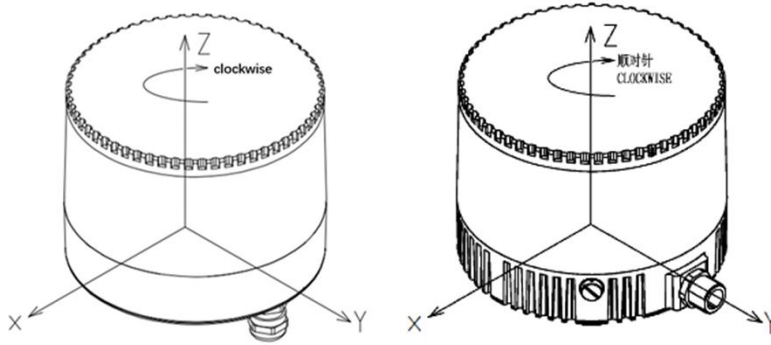
Figure 1.3 Coordinates & Scanning Direction (left: bottom; right: side)
