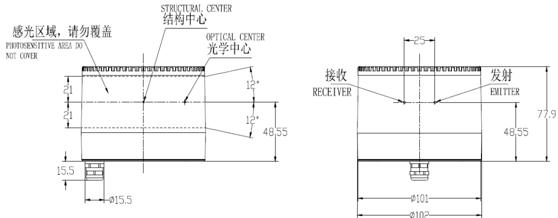
Figure 1.6 C8 Mechanical Drawing 1 (cable interface on the bottom) (unit: mm)
