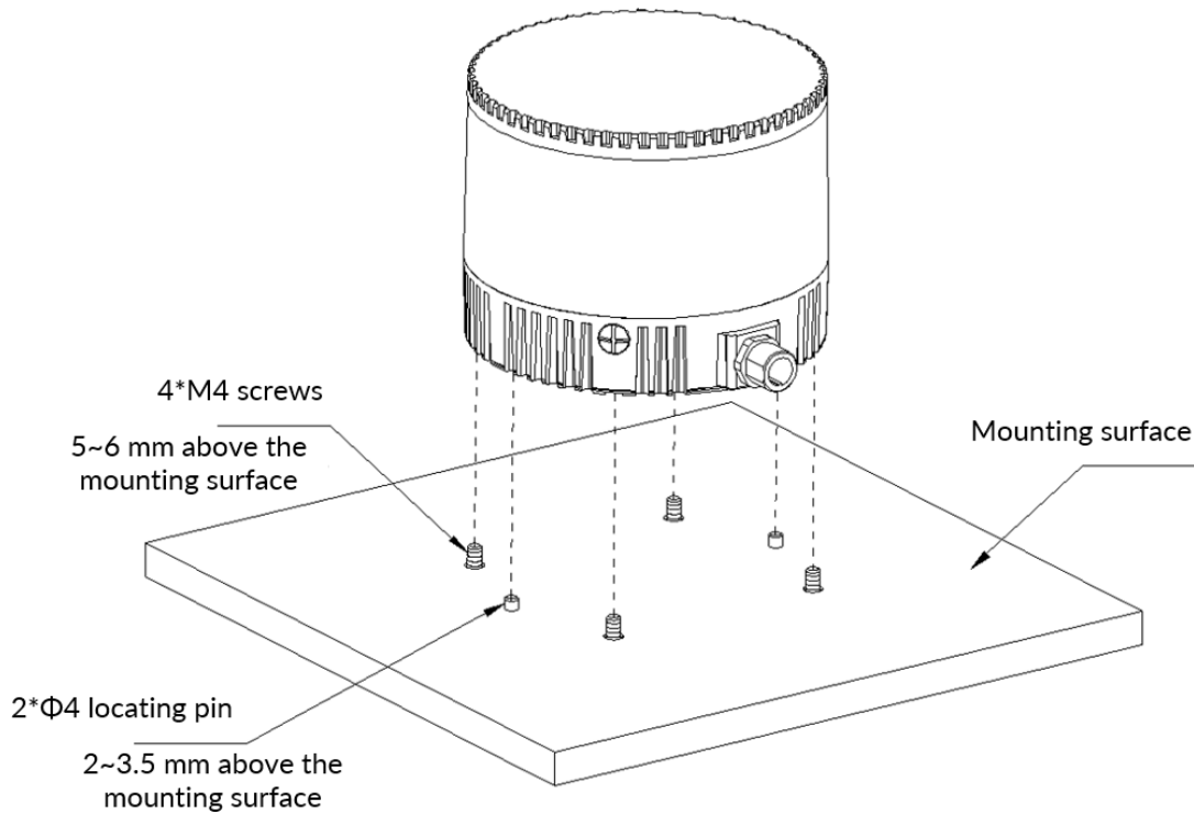
Figure 1.8 Lidar Mounting Reference Drawing
