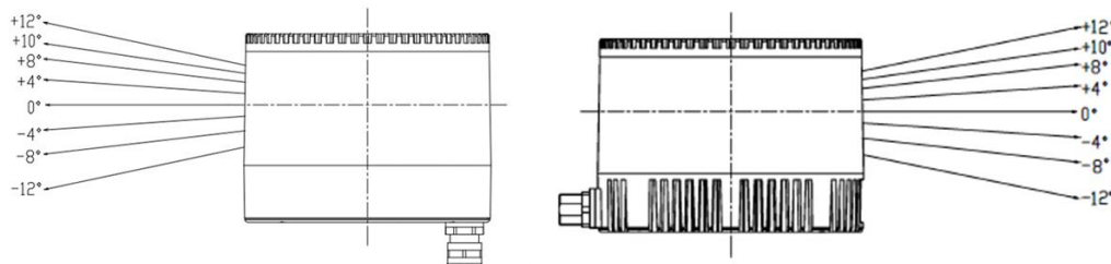
Figure 1.2 Laser Beam Distribution (left: bottom; right: side)
