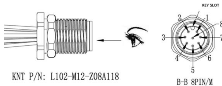
Figure 2.3 Cable Connector on the Side
