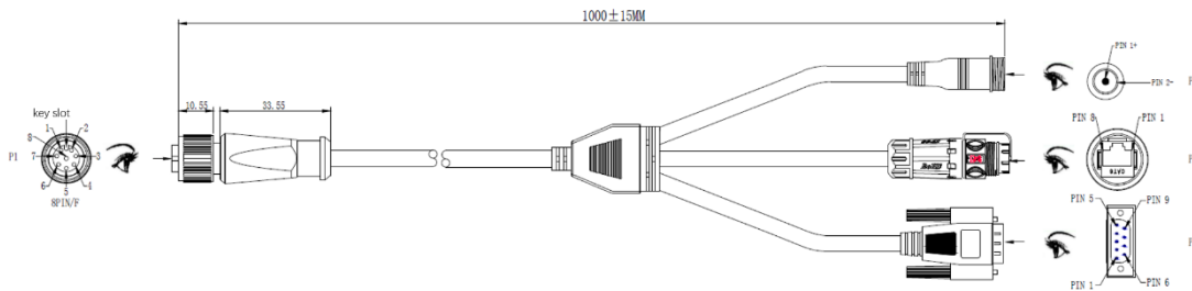
Figure 2.4 Adapter Cable
